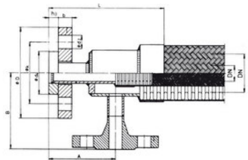
Note | Type DS - Double Shell Hose | dimensional sketch
