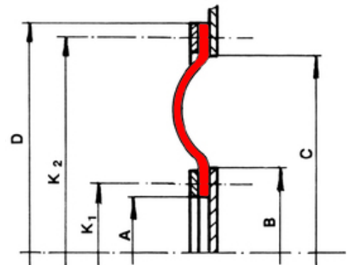
Note | Type 35 - Fabric Expansion Joint | dimensional sketch
