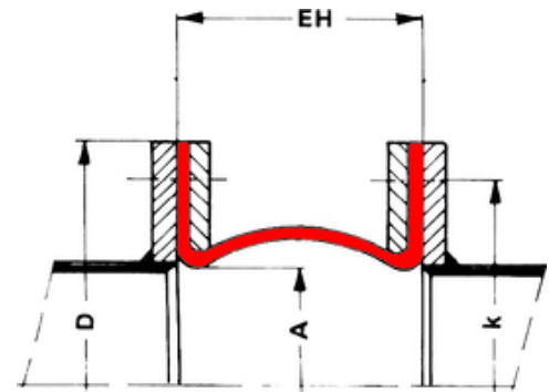
Note | Type 32 - Fabric Expansion Joint | dimensional sketch
