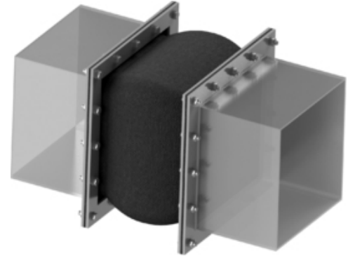
Note | Type 32 - Fabric Expansion Joint | 3D view
